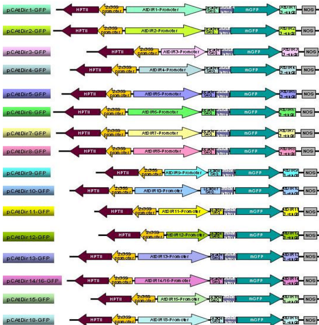
Figure 2. Schematic diagrams of dirigent promoter:: mgfp ::3' flanking fusion proteins.
